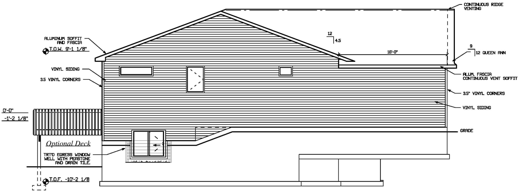
Left Elevation
