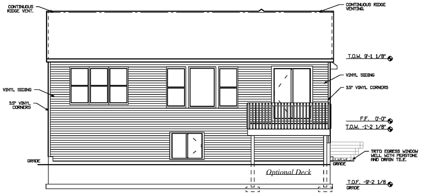
Rear Elevation
