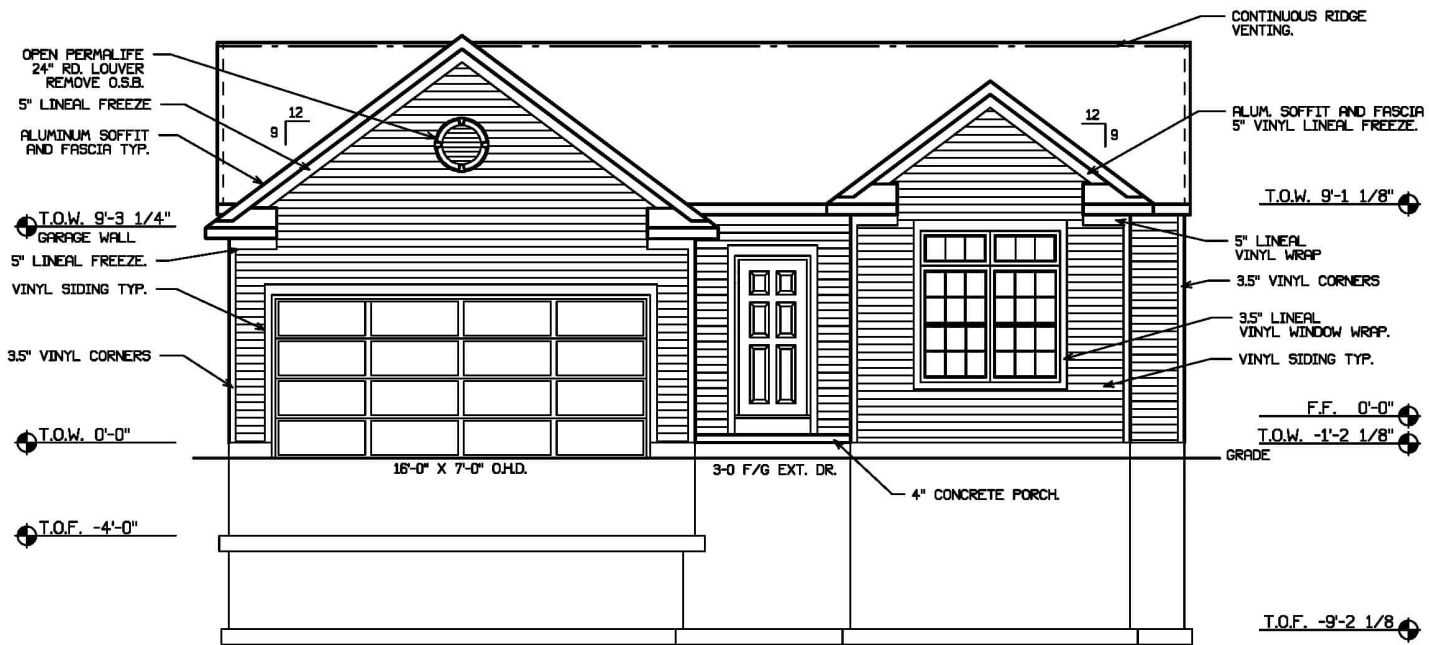
Front Elevation
