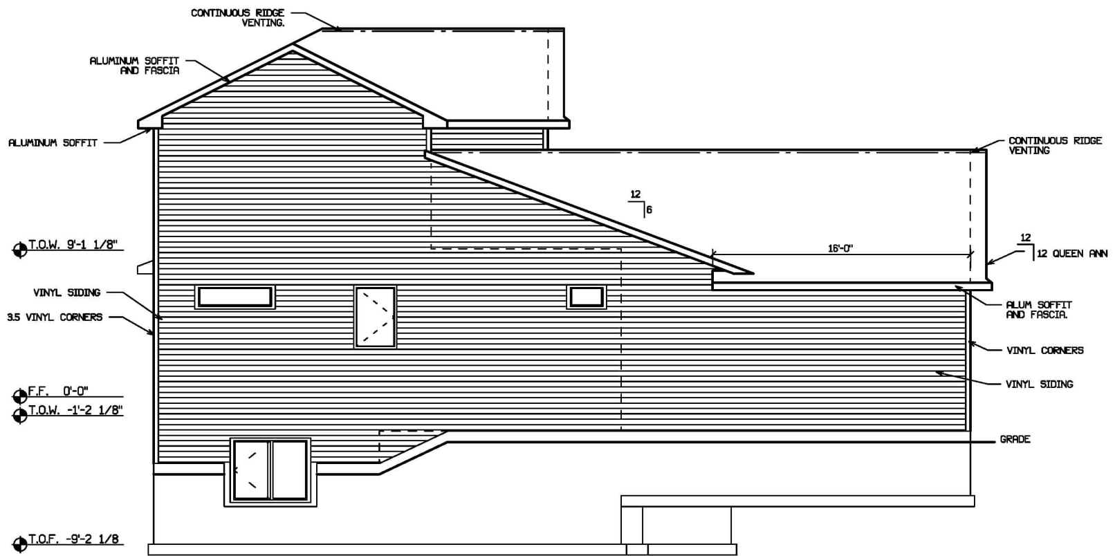
Left Elevation
