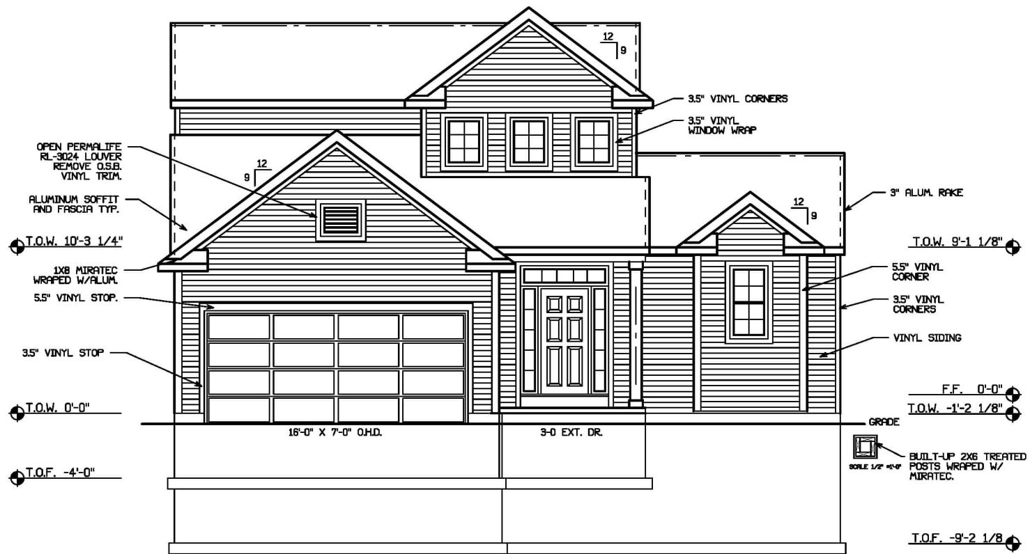
Front Elevation
