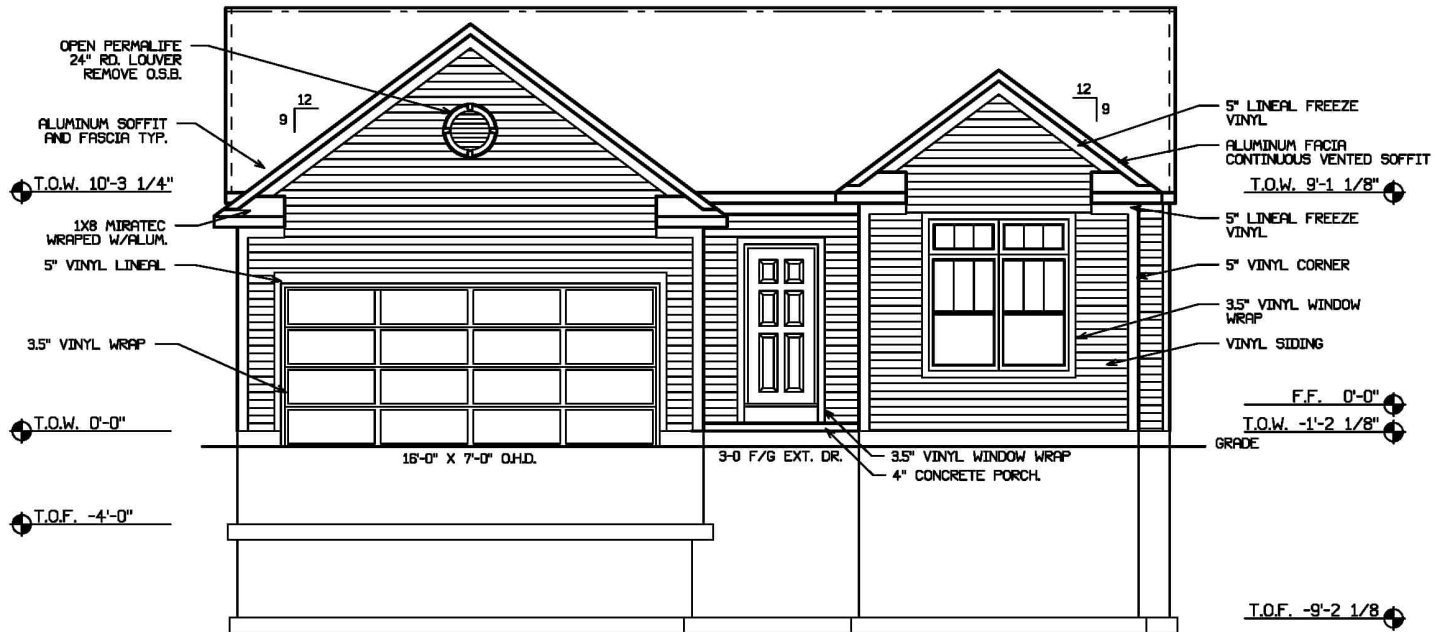
Front Elevation
