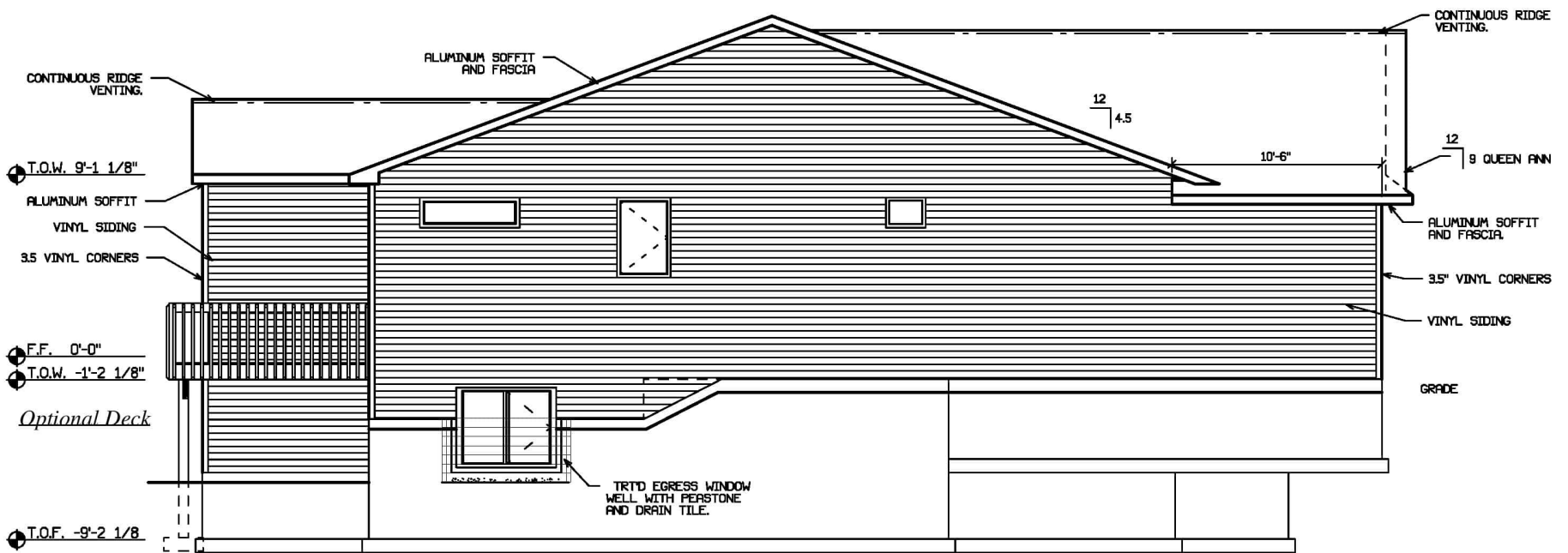
Left Elevation
