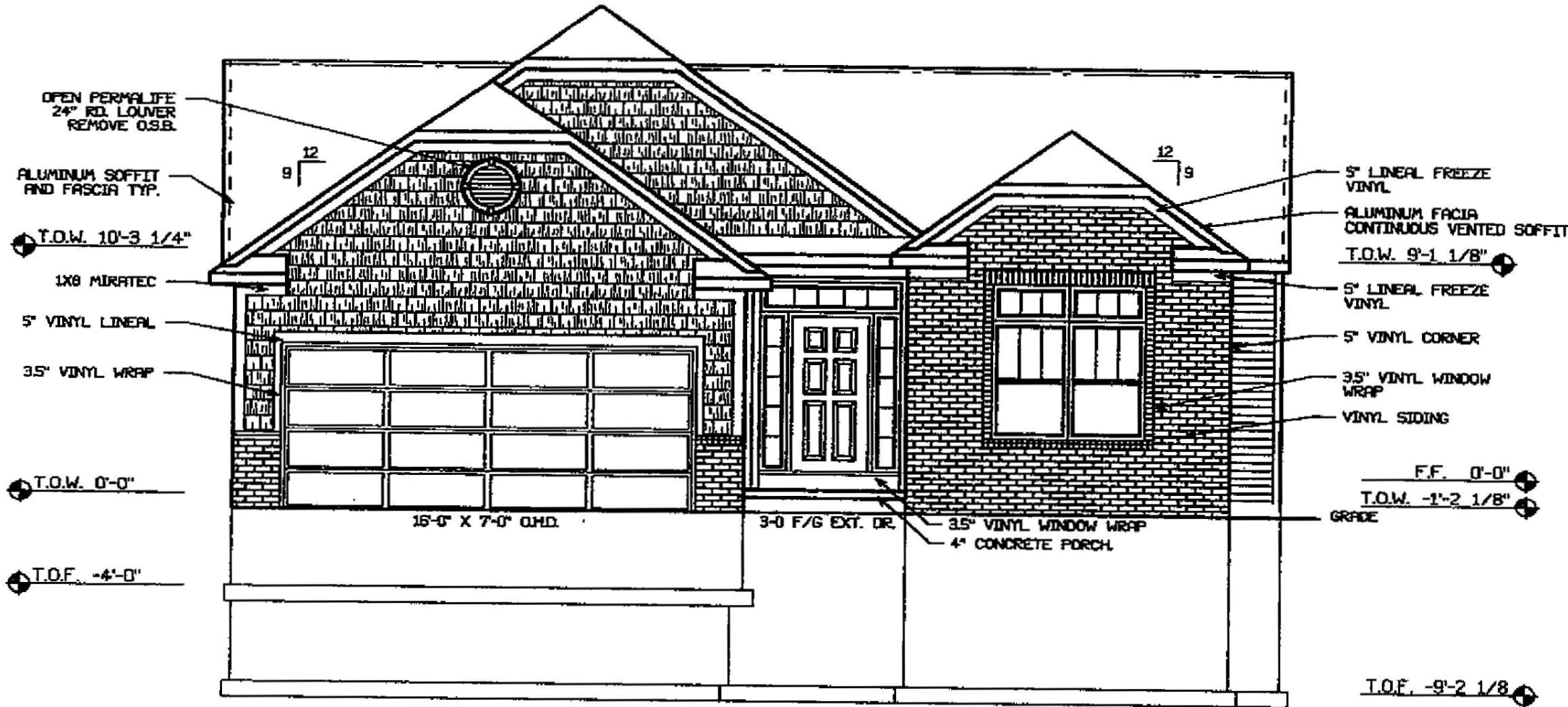
Front Elevation
