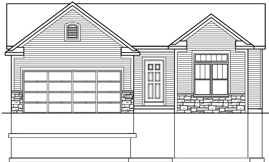
Base Front Elevation "A"
